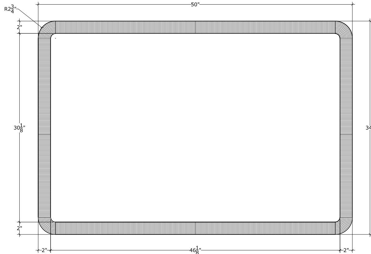
Front View
