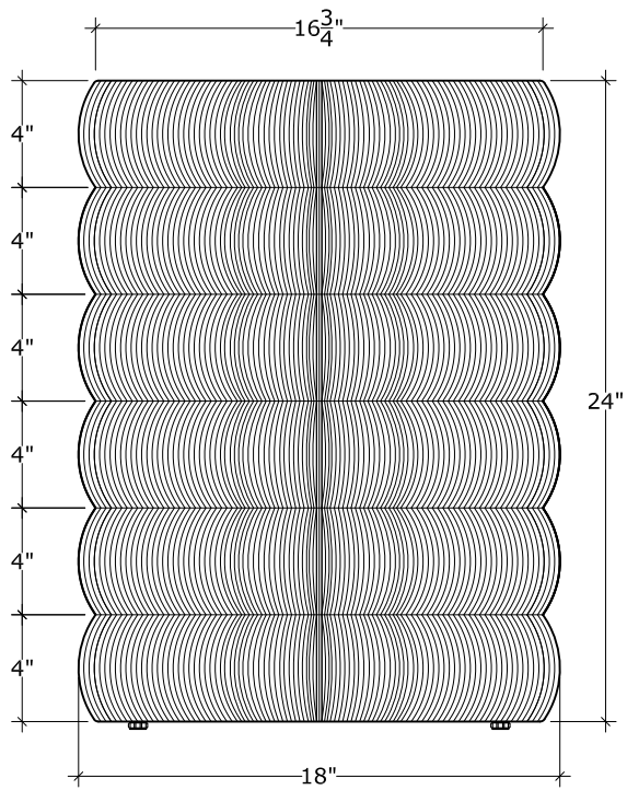
End View
